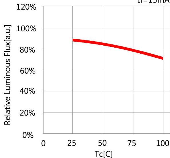
Temperature vs. Relative Luminous Flux I F =15mA
