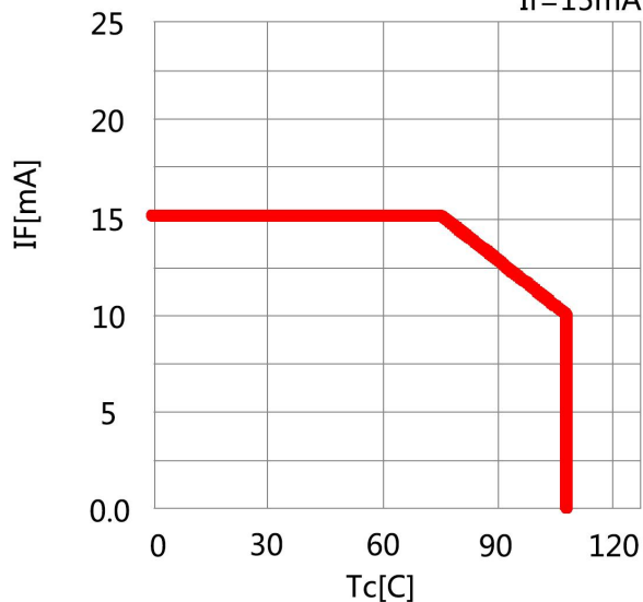
Temperature vs. Forward Current I F =15mA
