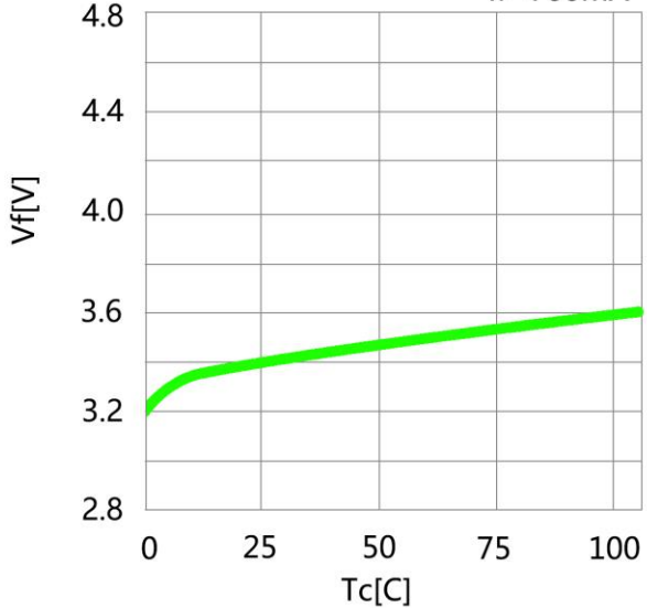
Case Temperature vs. Forward Voltage I_f=700\text{mA}
