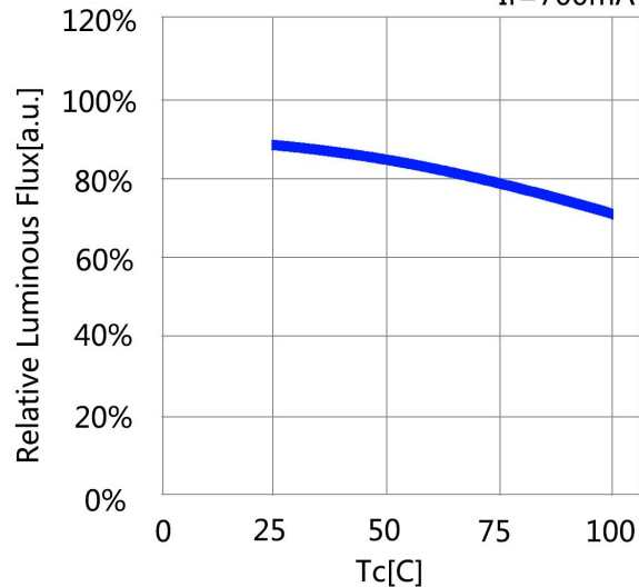
Temperature vs. Relative Luminous Flux If=700mA
