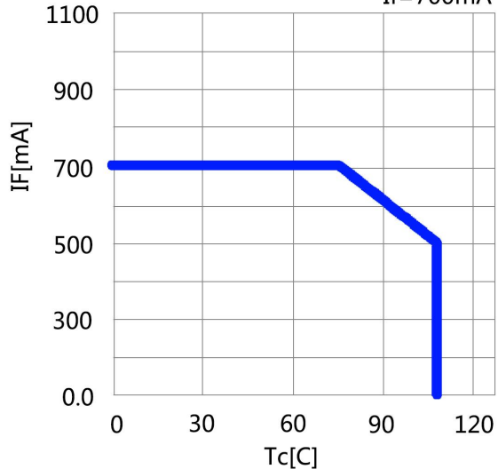
Temperature vs. Forward Current If=700mA
